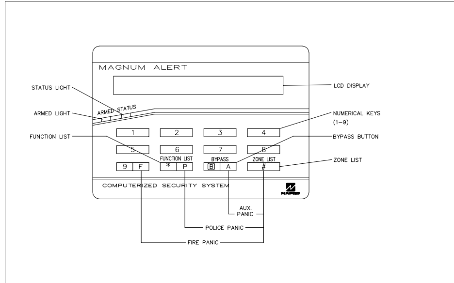
Keypad controls.
